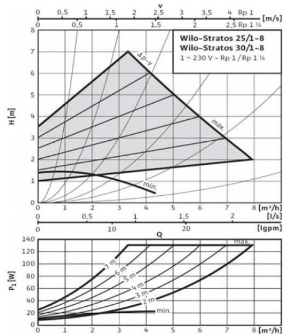
Δp-variable
