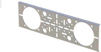
1062947 Uponor Mounting Bracket M7 c/c 80 mm 1062948 Uponor Mounting Bracket M7 c/c 150 mm 1062949 Uponor Mounting Bracket M7 c/c 160 mm
