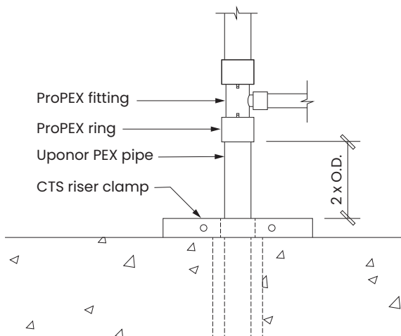
Figure 68: Riser clamp detail
