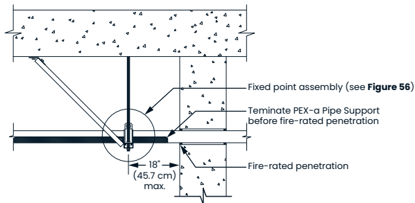
Figure 57: Fixed points near a fire-rated penetration (horizontal)
