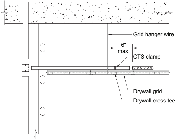
Figure 53: Supporting multiport tees on drywall grid
