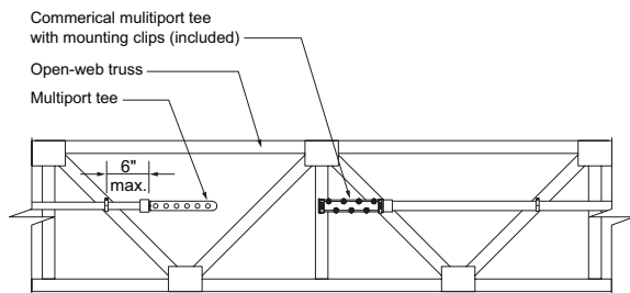
Figure 51: Supporting multiport tees on open-web wood trusses
