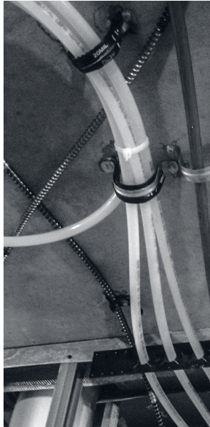
Figure 54: Proper bundling of Uponor PEX
