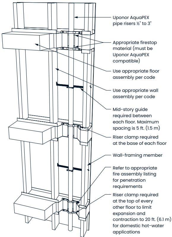
Figure 70: Domestic hot-water riser detail
