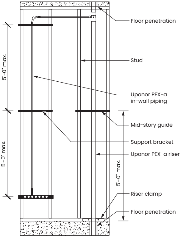
Figure 62: In-wall versus riser piping
