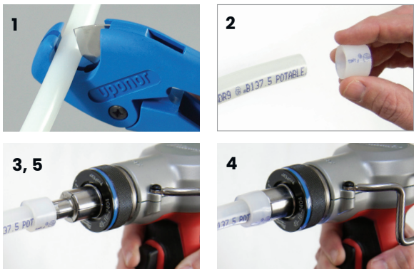
Figure 4: Expansion with Milwaukee M12, M12 FUEL, M18, and M18 FUEL 2" ProPEX expansion tools
