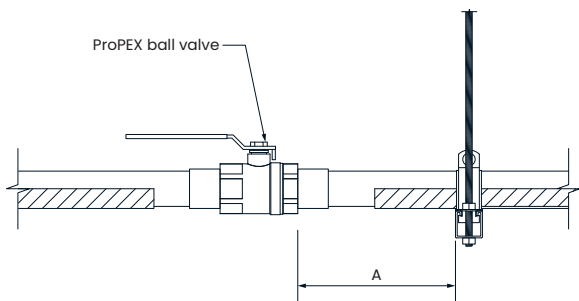
Figure 44: Supporting 1¼" to 2" ball valves
