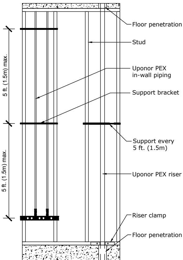
Figure 67: In-wall versus riser piping
