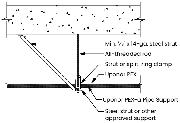
Figure 56: Fixed point
