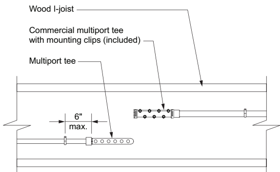
Figure 50: Supporting multiport tees on wood I-joists
