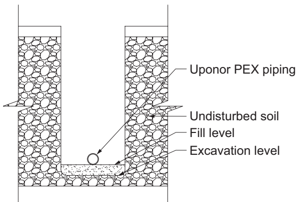
Figure 82: Good soil conditions — If the trench is dug smoothly, install the piping directly on the prepared bottom. The bottom must be flat with no hollows, lumps or rocks.
