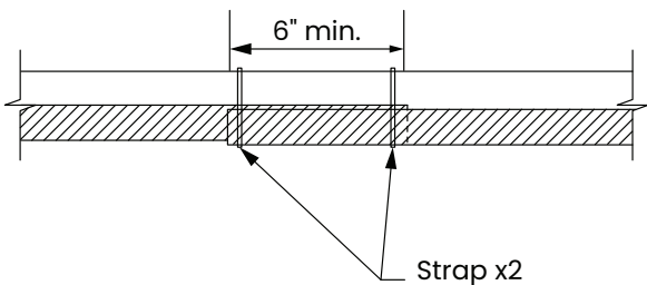
Figure 48: Strapping overlaps
