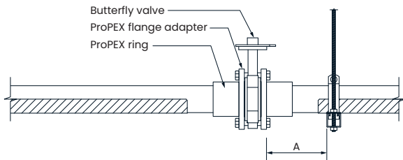
Figure 61: Supporting 2½" to 3" butterfly valves
