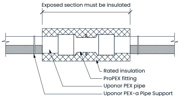
Figure 59: PEX-a Pipe Support installations in ASTM E84 applications
