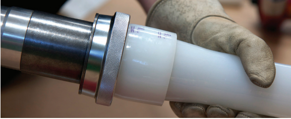
Figure 25: Expand to shoulder
