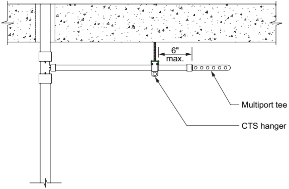
Figure 52: Supporting multiport tees in suspended applications
