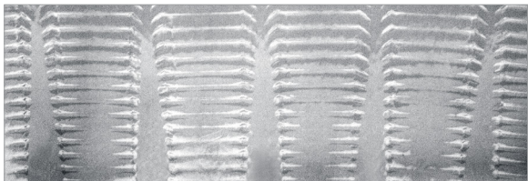
Figure 36: Expansion without proper rotation
