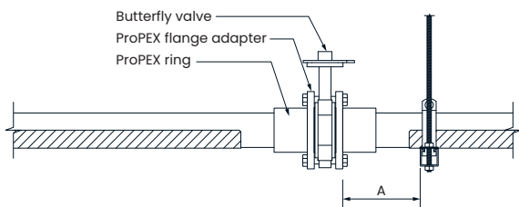
Figure 45: Supporting 2½" to 3" butterfly valves
