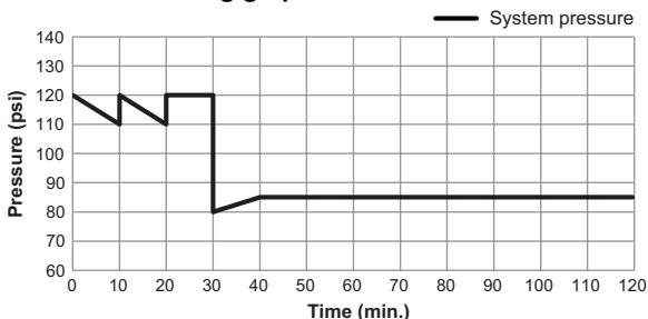
Figure 84: Pressure testing graph
