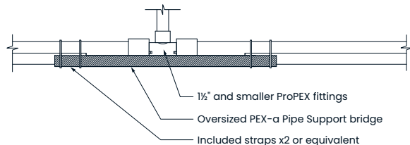
Figure 58: Fitting bridge
