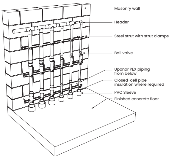
Figure 78: Mechanical room transition (below-grade piping)
