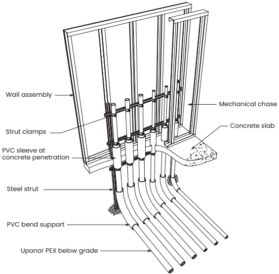
Figure 79: Wet-wall chase transition (below-grade piping)
