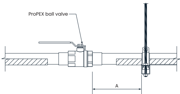
Figure 60: Supporting 1¼" to 2" ball valves
