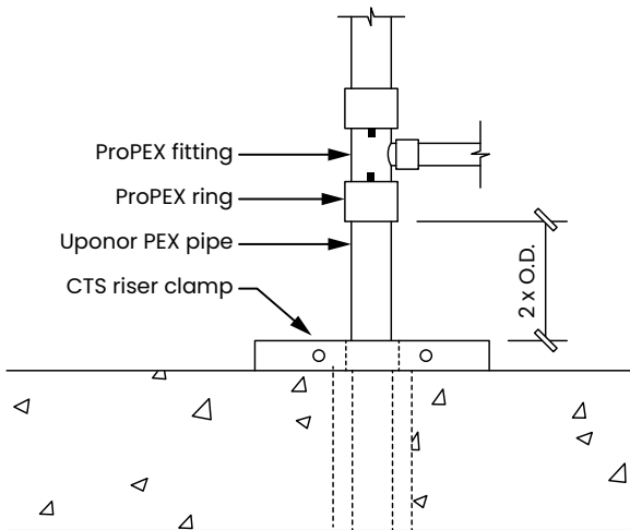
Figure 66: Clamp distance example
