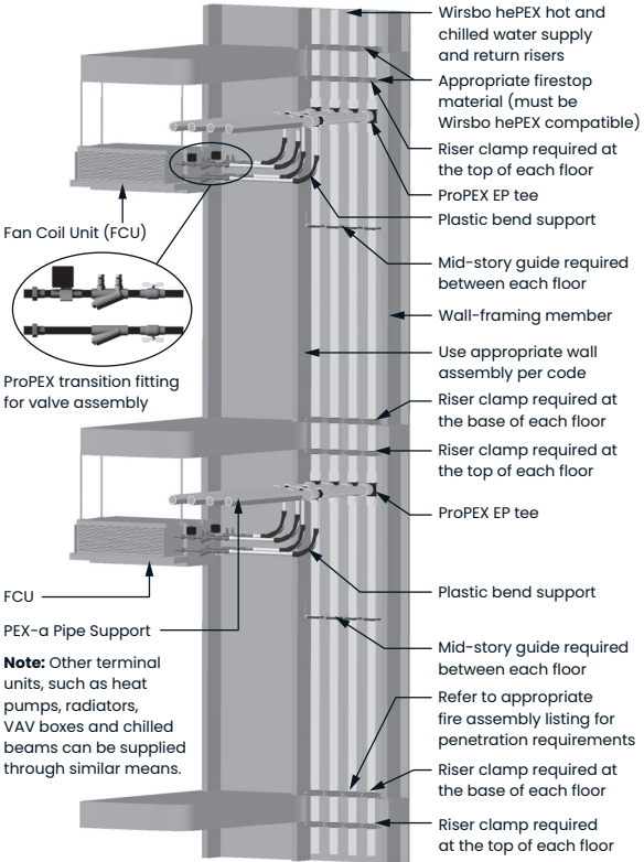
Figure 69: Hydronic piping riser detail
