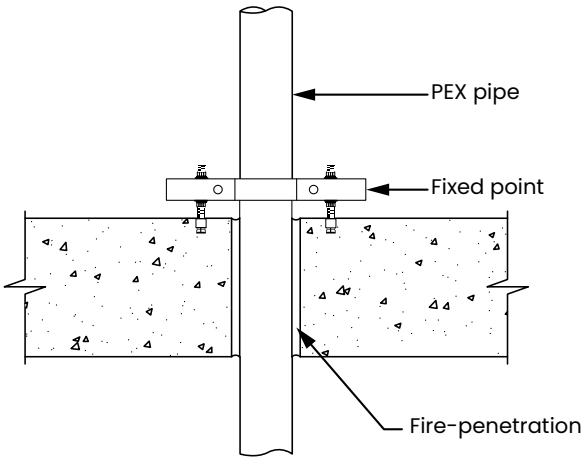
Figure 63: Fixed point example 1 (vertical)
