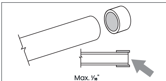
Figure 32: Slide the expanded ring over the end of the piping
