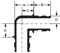
Brass elbow
