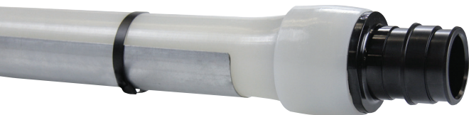
Figure 46: Uponor PEX-a Pipe Support with nylon strapping
