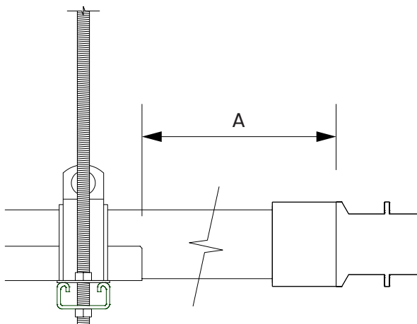
Figure 47: Minimum distance to fitting
