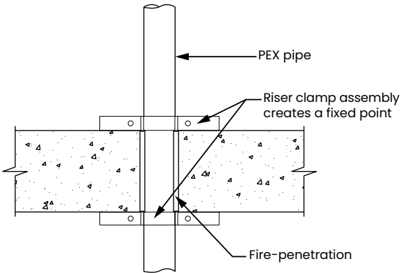
Figure 64: Fixed point example 2 (vertical)
