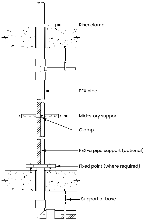
Figure 65: PEX riser detail
