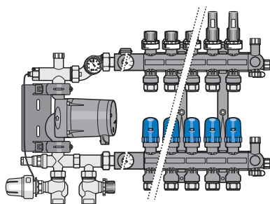
Uponor PRO 1" Manifold with Uponor Push 23A
