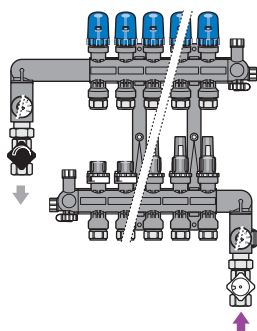
Connection both sides from below
