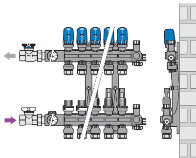
Lateral connection
