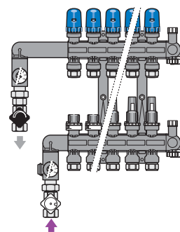
Connection one side from below
