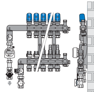
With heat meter - installed vertically
