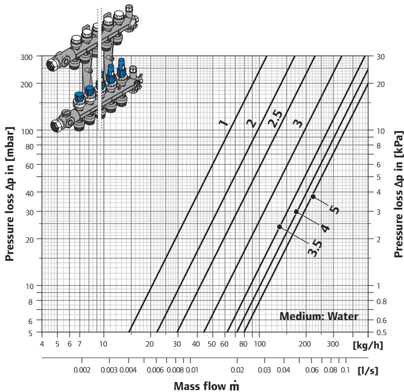
Valve presetting diagram (number of turns) for regulating and balancing valves in Uponor PRO 1" Manifolds
