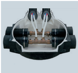
Uponor Ecoflex chamber
