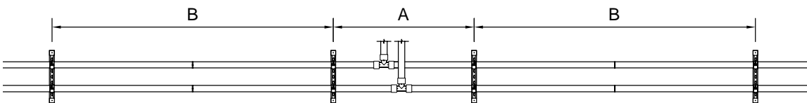
Figure 6-15: PEX-a Pipe Support with fittings
