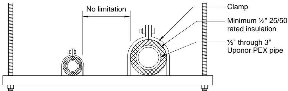
Figure 3-19: QAI P321-1
