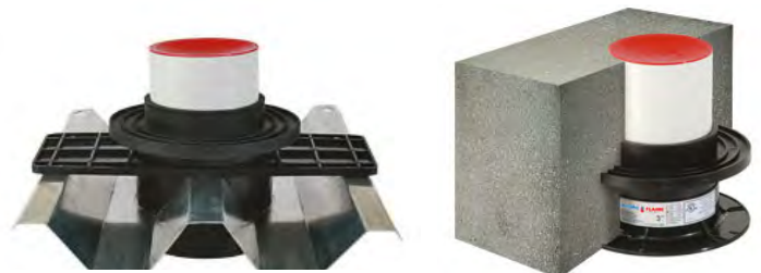
Figure 3-17: Cast-in-place sleeves
