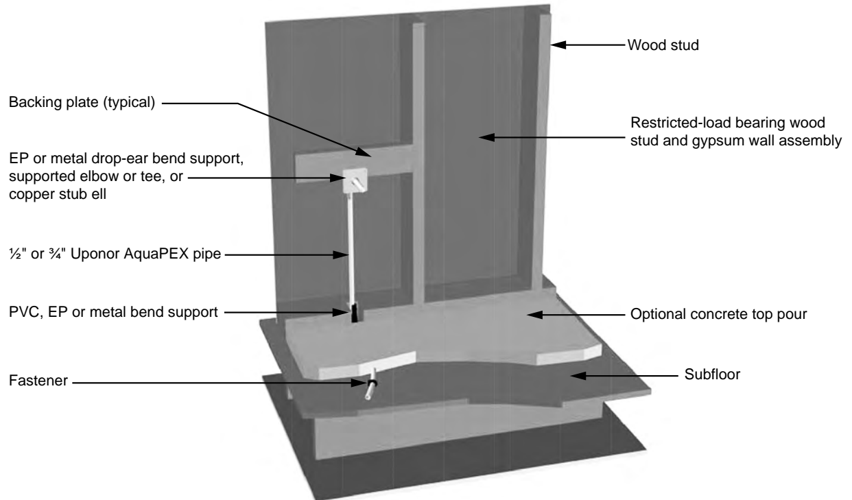
Figure 3-6: fixture detail 2
