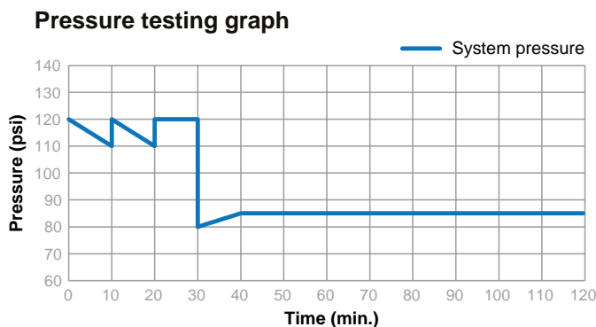
Figure 6-49: Pressure testing graph
