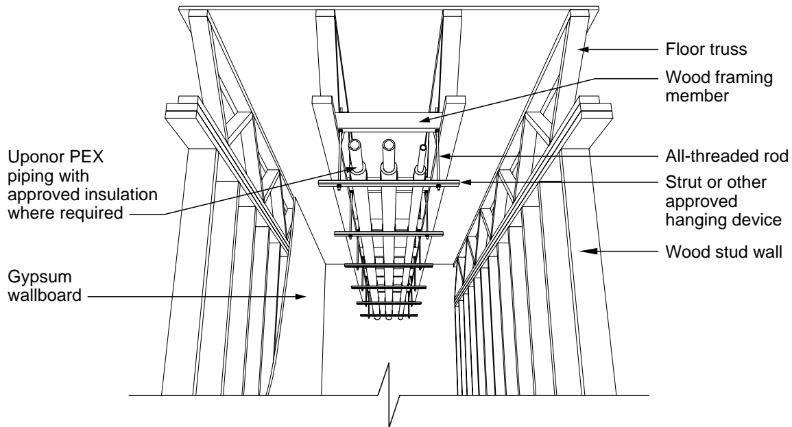
Figure 6-31: Hallway/corridor detail
