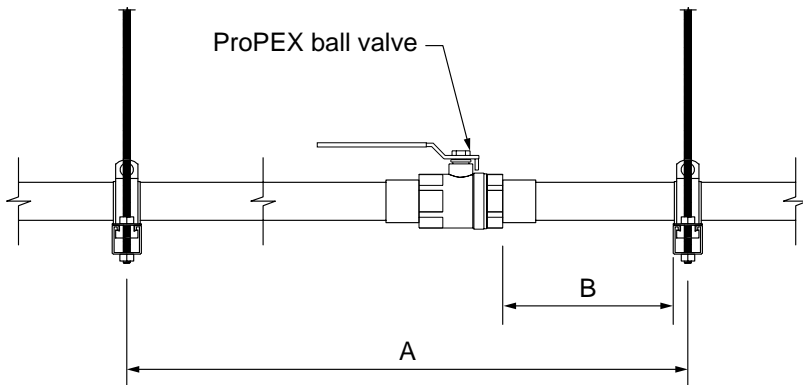
Figure 6-10: Supporting 1 1/4" to 2" ball valves
