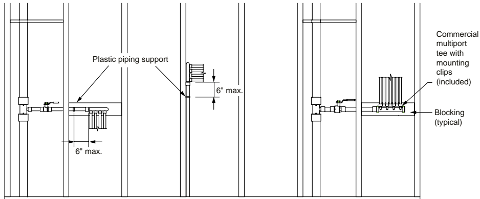
Figure 6-25: In-wall supports for multiport tees
