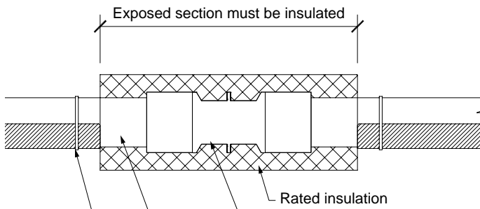
Figure 6-23: PEX-a Pipe Support installations in ASTM E84 applications
