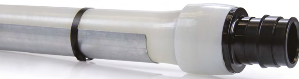
Figure 6-13: Uponor PEX-a Pipe Support with nylon-coated, stainless-steel strapping
