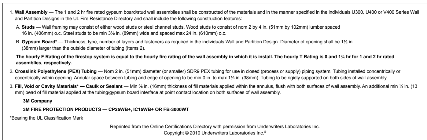
Figure 3-16: Assembly criteria
