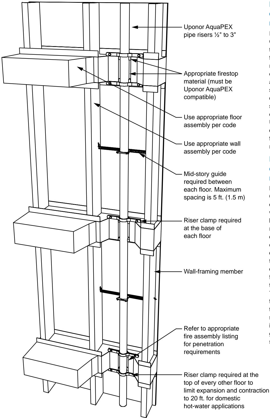
Figure 6-40: Hot-water risers
