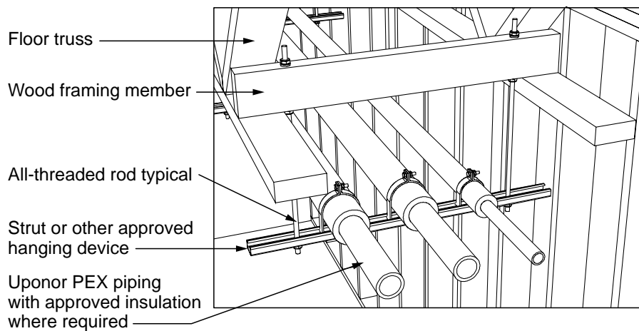
Figure 6-32: Hanger detail
