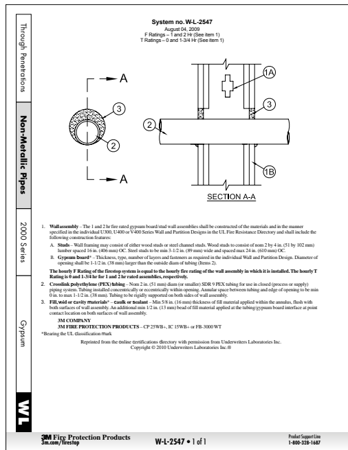
Figure 3-14: Fire assembly document
