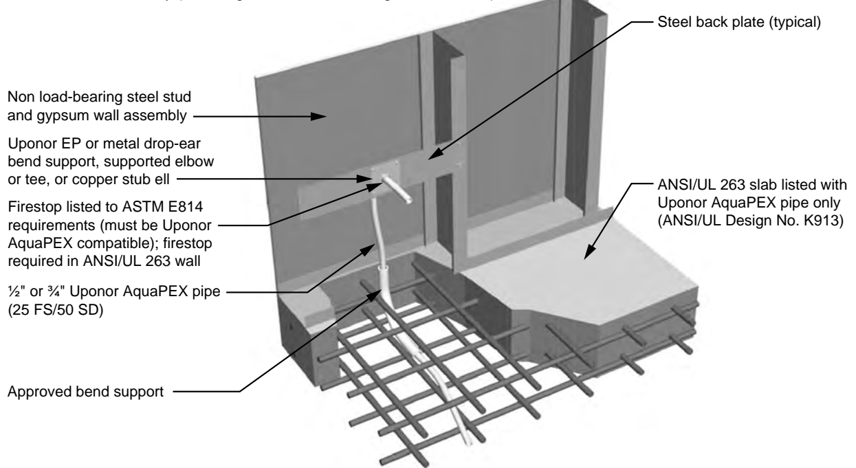
Figure 3-8: Fixture detail
