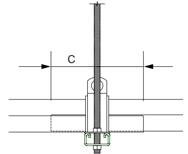
Figure 6-18: Minimum overlap
