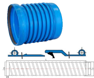
Ø1200-2500:
